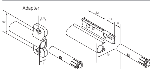
Magnet-Pin / Magnetic Pin
